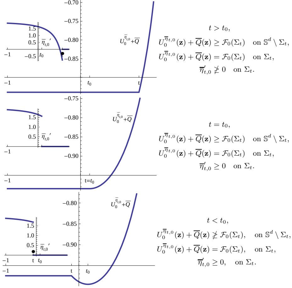
FIGURE 2. The weighted logarithmic potential of \bar{\eta}_{t,0} for t > t_0 , t = t_0 , and t < t_0 versus altitude \xi of \mathbf{z} for d = 2 , s = 0 , q = 1 , and R = 2 , cf. Theorem 1.17. Insets show the respective density \bar{\eta}'_{t,0} . The dot indicates the component on the boundary of \Sigma_t .
