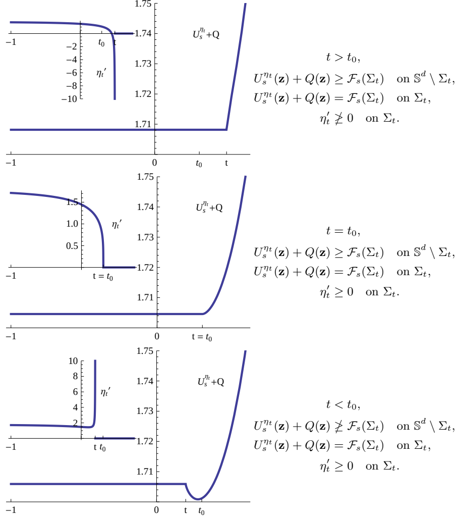
FIGURE 1. The weighted s -potential of \eta_t for t > t_0 , t = t_0 , and t < t_0 versus altitude \xi of \mathbf{z} for d = 2 , s = 1/2 , q = 1 , and R = 3/2 , cf. Theorems 1.11 and 1.13. Insets show the respective density \eta'_t .
