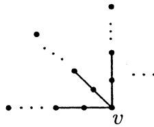
Figure 1: The d -pode R(c_1, \dots, c_d) .
