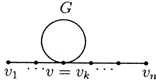
Figure 3: The graph P(n, k, G, v) .
