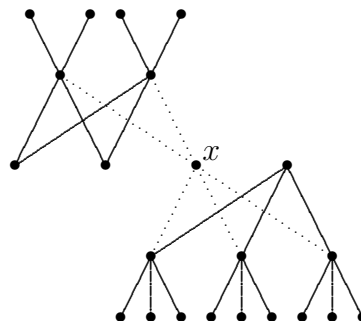
Figure 3b: N_2(x) in \text{DL}(3, 2)
