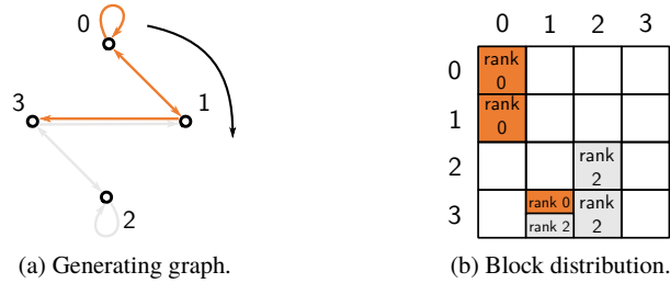
Fig. 2 Distribution of the system matrix blocks among four processes.
