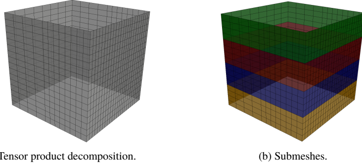
Fig. 1 Sample space-time boundary decompositions for Q = (0, 1)^3 .
