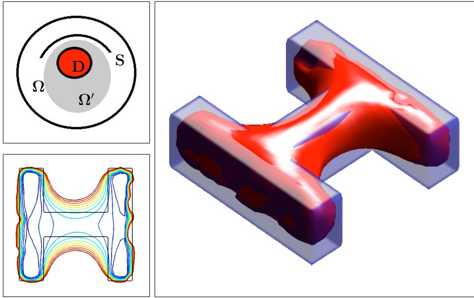
FIGURE 1. Top-left: Sketch of the geometry. Bottom-left: Isolin plot of the reconstruction c_n (red) and the true object (blue) at the plane \{(x, y, 0.4)\} . Right: Isosurface of the reconstruction c_n (red) and the domain D of the scattering object (blue).
