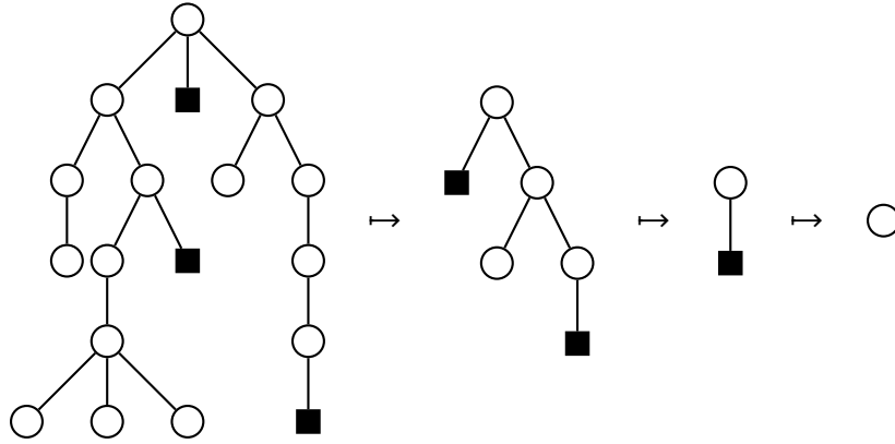
FIGURE 3. Illustration of the reduction operator \rho , \blacksquare marks the rightmost leaves in the branches attached to the root.
