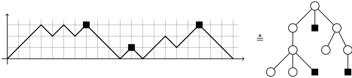
FIGURE 1. Bijection between Dyck paths with odd returns to zero and Catalan–Stanley trees. ■ marks all peaks before a descent to the x -axis and all rightmost leaves in the branches attached to the root, respectively.
