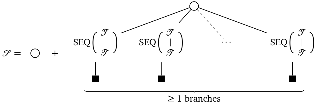
FIGURE 2. Symbolic specification of the combinatorial class \mathcal{S} of Catalan–Stanley trees. Nodes represented by \blacksquare are marked by the variable t , all other nodes are marked by z .
